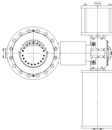
Valve with horizontal shaft
